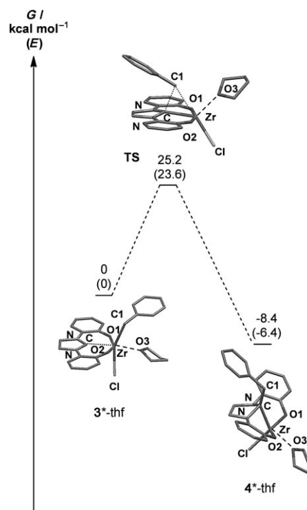
Figure 4. Energy profile of the rearrangement of the NHC–Zr THF adduct 3*-thf computed at the BP3LYP/SDD(Zr),6-31G**(other atoms) level of theory. Free energies ( G ), at 25 °C including ZPE correction are expressed in kcal mol -1 , total energies ( E ) are reported into brackets. Hydrogen atoms are omitted for clarity.
