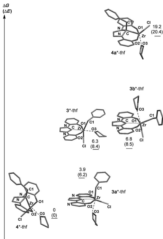
Figure 3. Gibbs free energies ( \Delta G ), and total energies ( \Delta E ; in brackets) of the calculated DFT structures 4*-thf (versus 3*-thf ) and their respective isomers in kcal mol -1 ( 4a*-thf , 3a*-thf , and 3b*-thf ). Hydrogen atoms are omitted for clarity.
